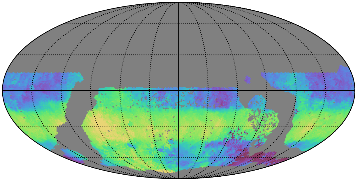
too_elab_r128_d2_gz_v3.4_10yrs WFD u band: Median HA
