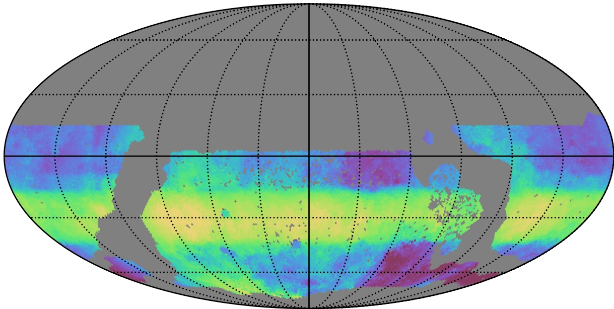
too_elab_r128_d2_gz_v3.4_10yrs WFD r band: Median HA
