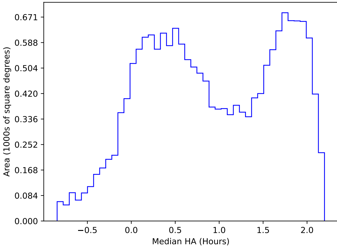
too_elab_r128_d2_gz_v3.4_10yrs WFD r band: Median HA
