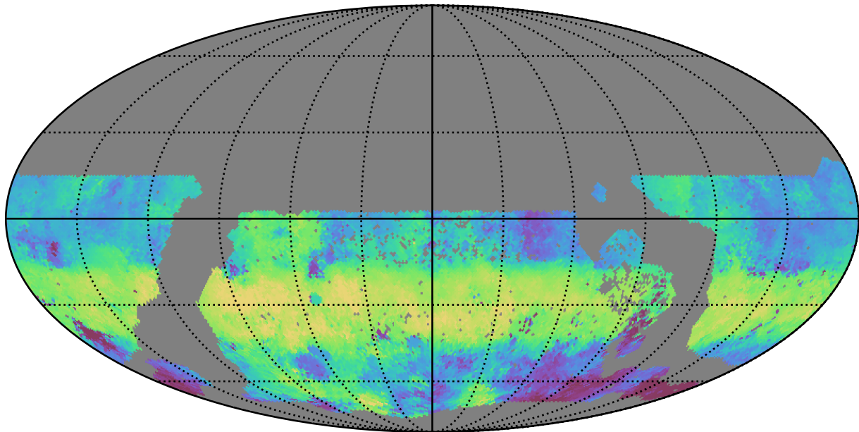
too_elab_r128_d2_gz_v3.4_10yrs WFD g band: Median HA
