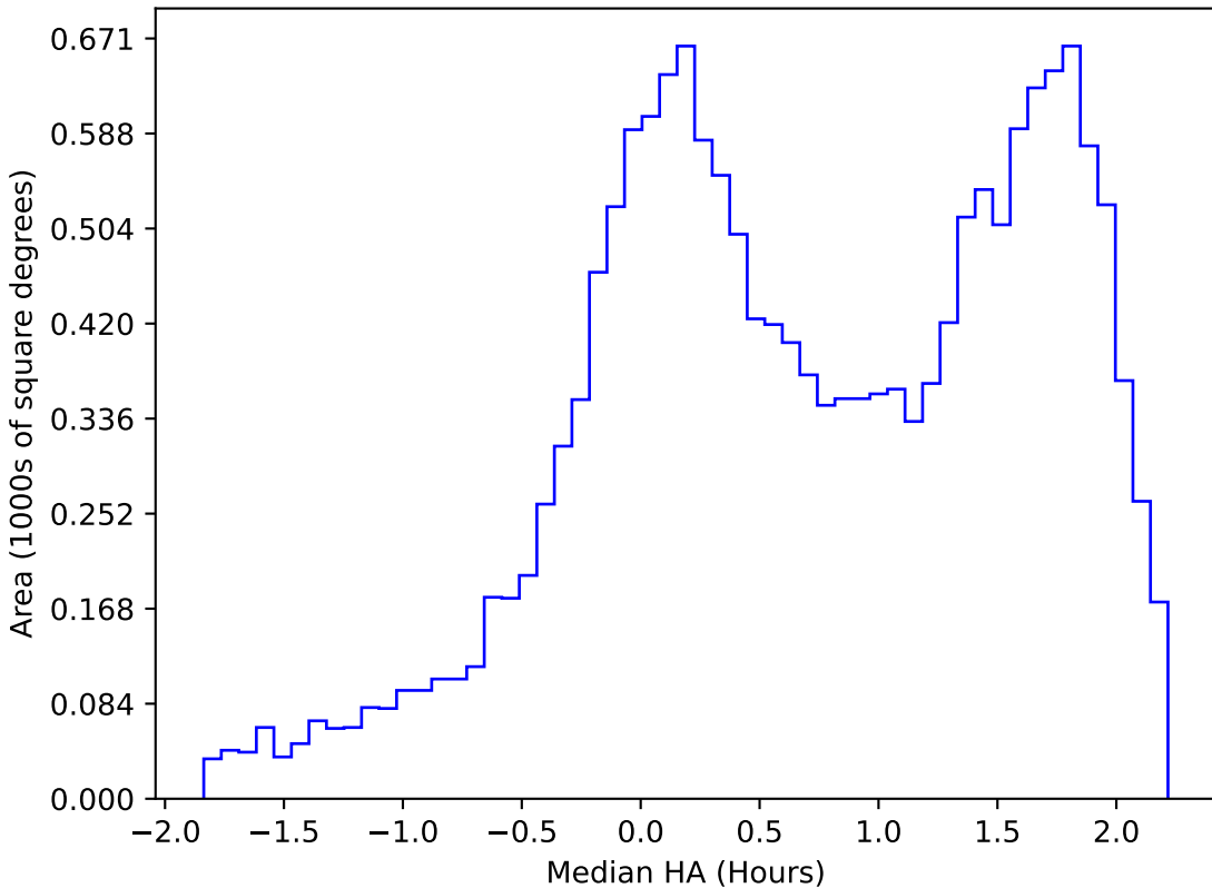
too_elab_r128_d2_gz_v3.4_10yrs WFD g band: Median HA
