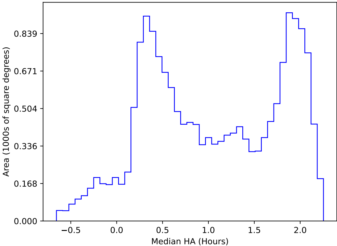
too_elab_r128_d2_gz_v3.4_10yrs WFD all bands: Median HA
