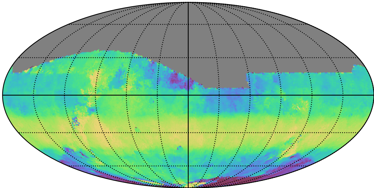
too_elab_r128_d2_gz_v3.4_10yrs All sky z band: Median HA
