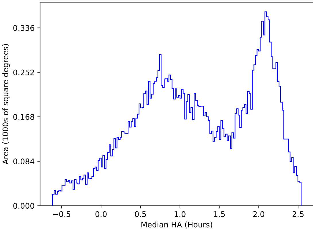
too_elab_r128_d2_gz_v3.4_10yrs All sky y band: Median HA
