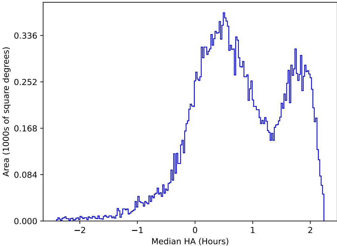
too_elab_r128_d2_gz_v3.4_10yrs All sky r band: Median HA
