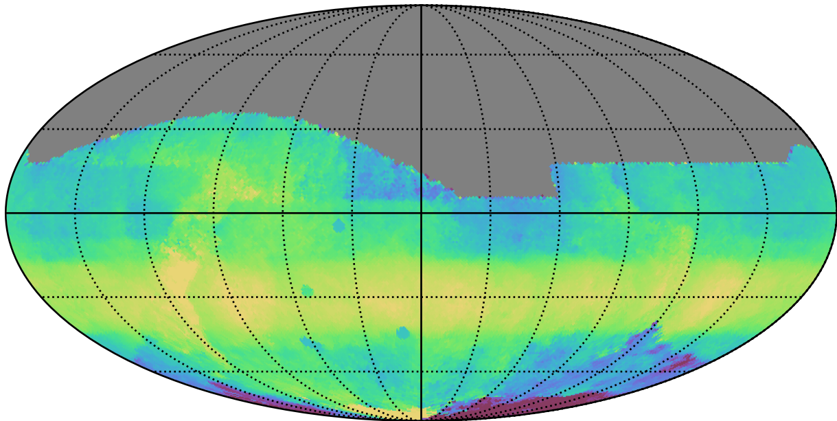
too_elab_r128_d2_gz_v3.4_10yrs All sky i band: Median HA
