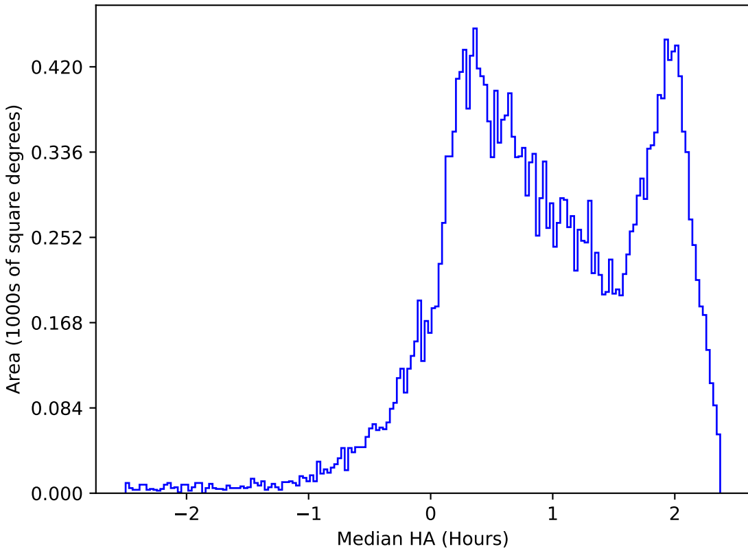
too_elab_r128_d2_gz_v3.4_10yrs All sky i band: Median HA
