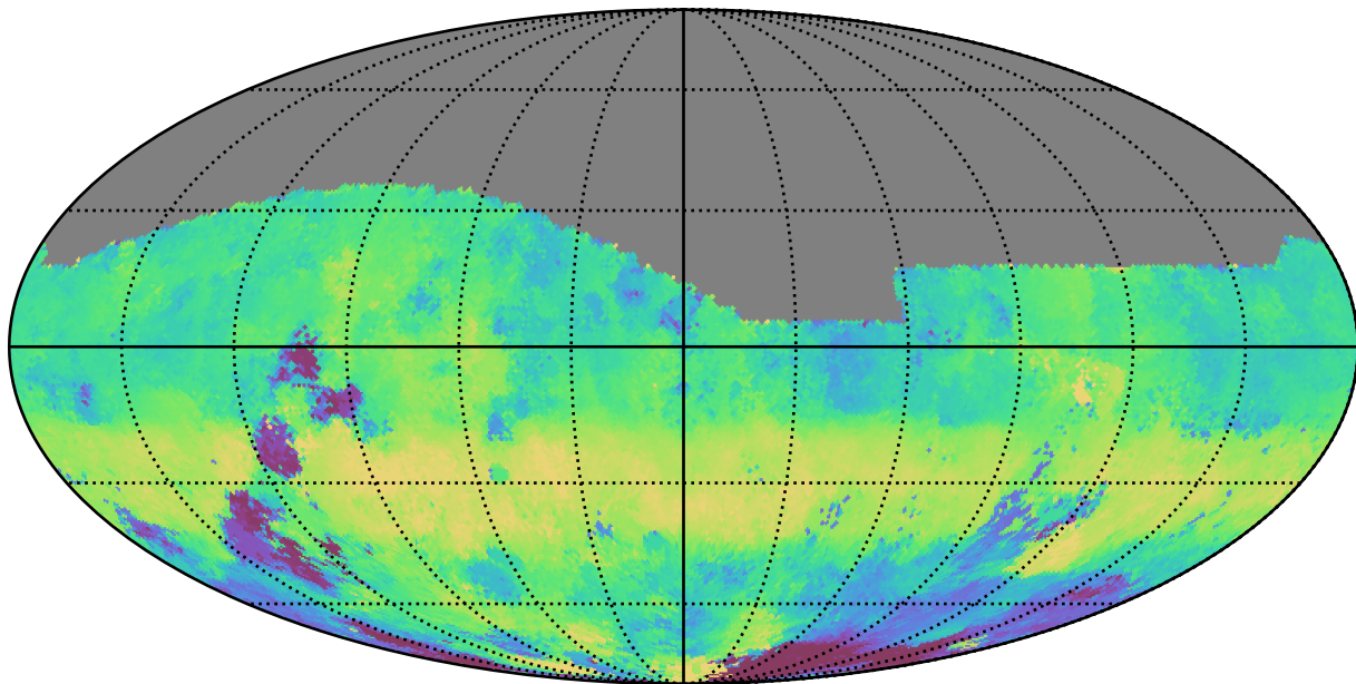
too_elab_r128_d2_gz_v3.4_10yrs All sky g band: Median HA
