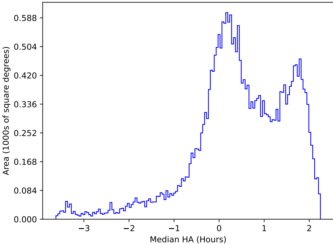
too_elab_r128_d2_gz_v3.4_10yrs All sky g band: Median HA
