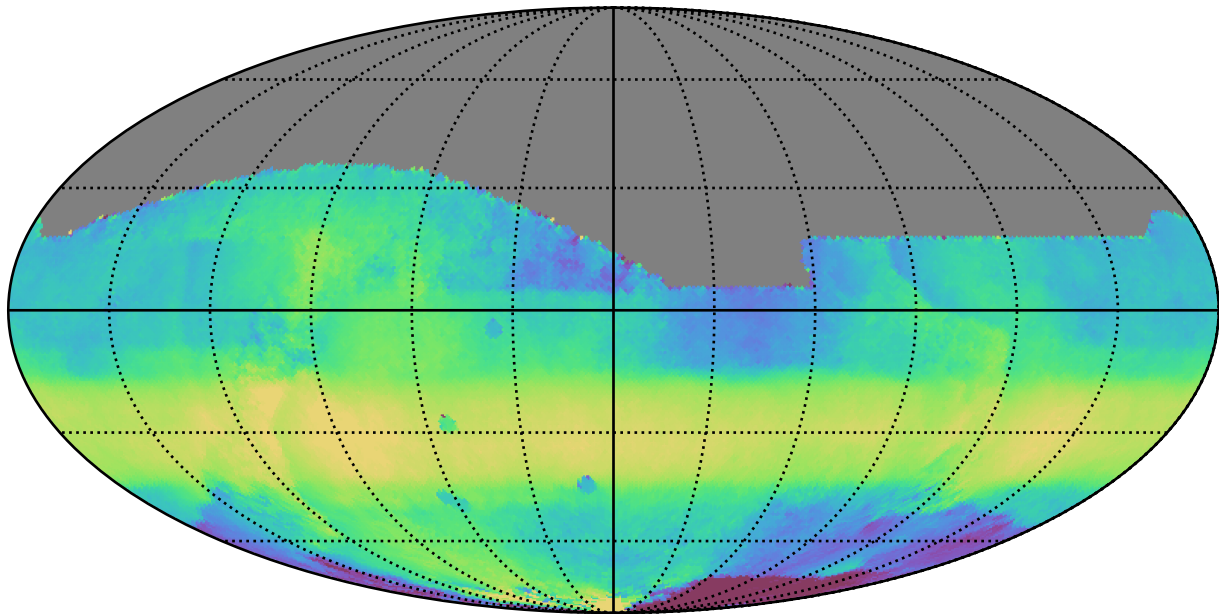
too_elab_r128_d2_gz_v3.4_10yrs All sky all bands: Median HA
