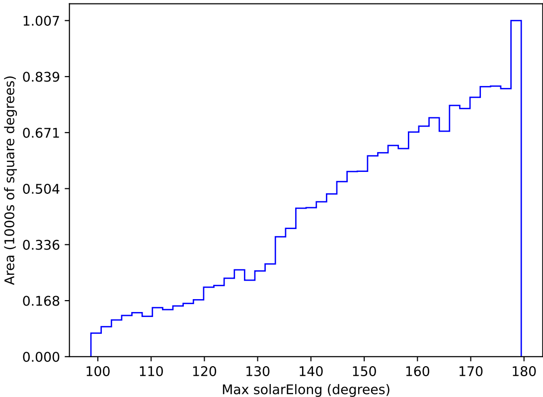
too_elab_r128_d2_gz_v3.4_10yrs WFD z band: Max solarElong
