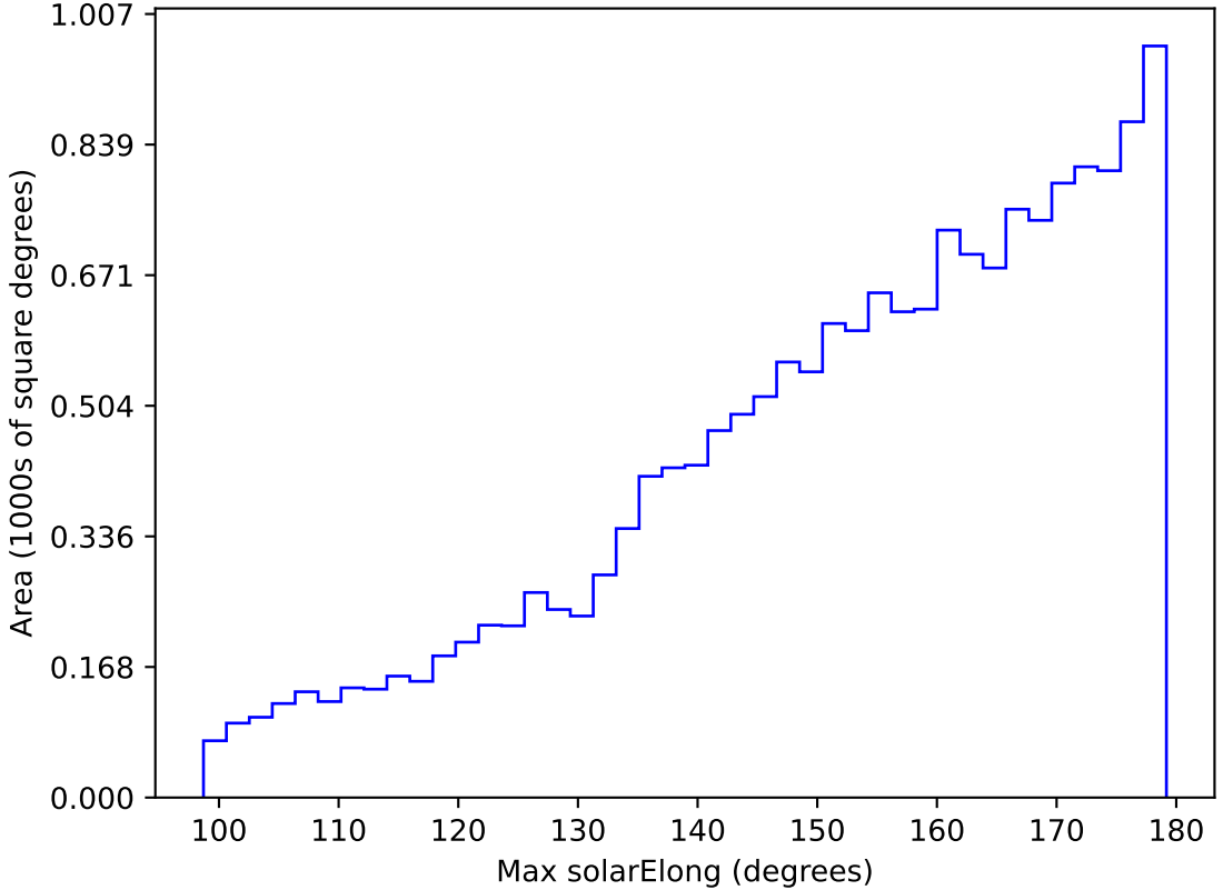
too_elab_r128_d2_gz_v3.4_10yrs WFD y band: Max solarElong
