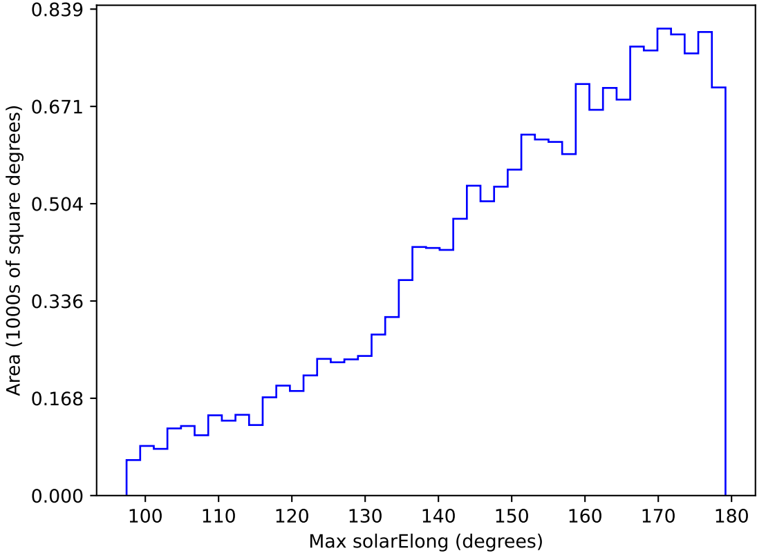
too_elab_r128_d2_gz_v3.4_10yrs WFD u band: Max solarElong
