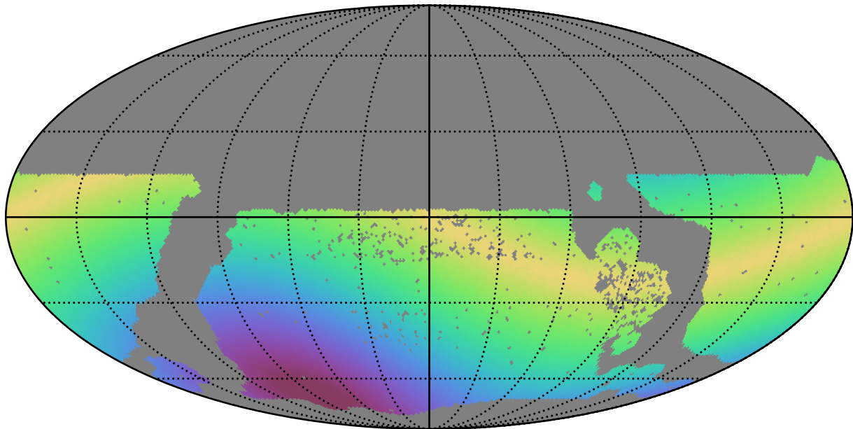
too_elab_r128_d2_gz_v3.4_10yrs WFD r band: Max solarElong
