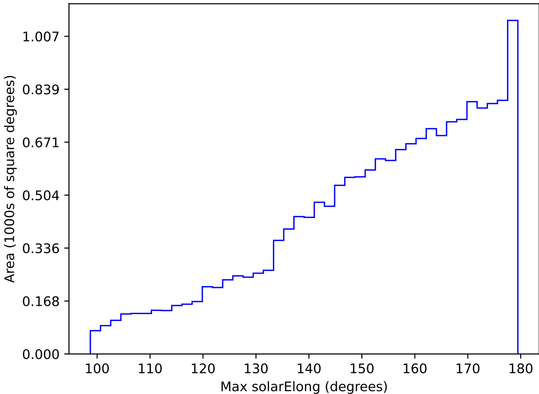
too_elab_r128_d2_gz_v3.4_10yrs WFD i band: Max solarElong
