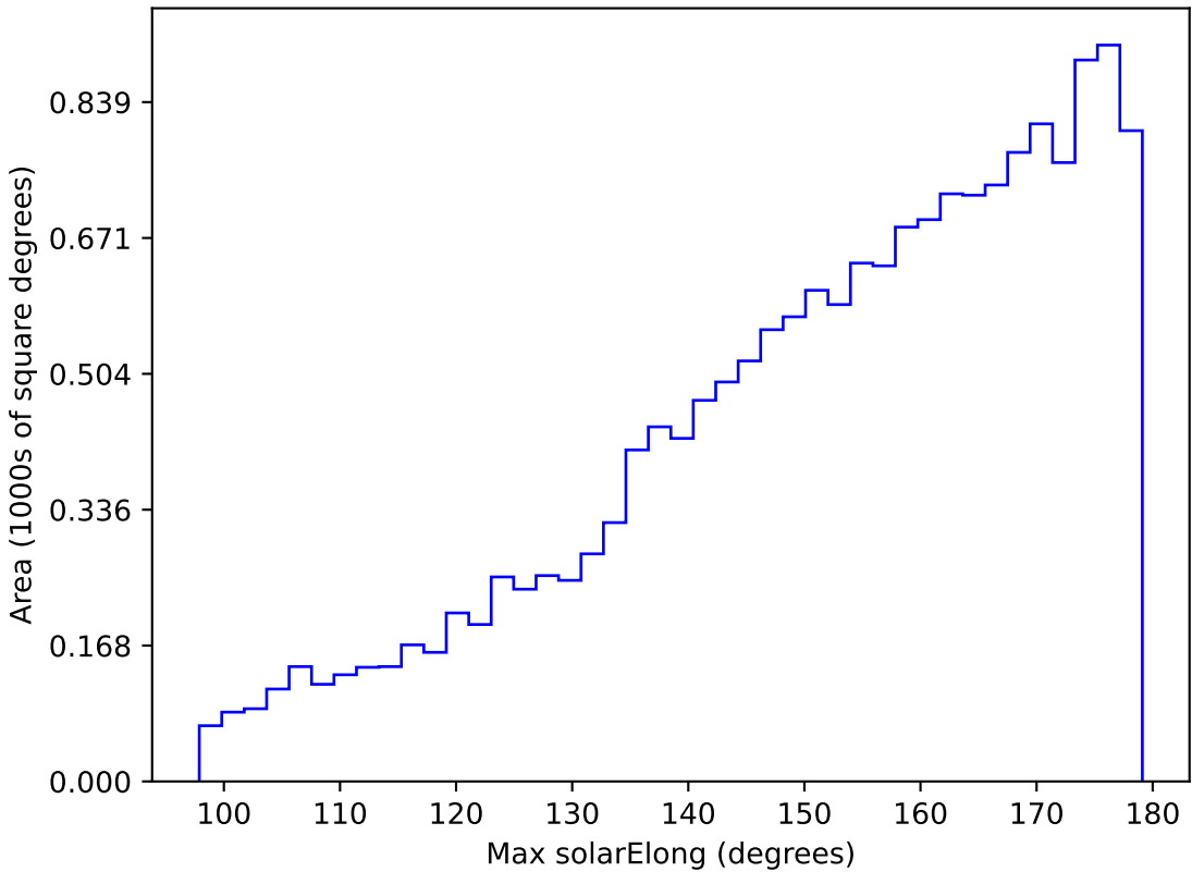
too_elab_r128_d2_gz_v3.4_10yrs WFD g band: Max solarElong
