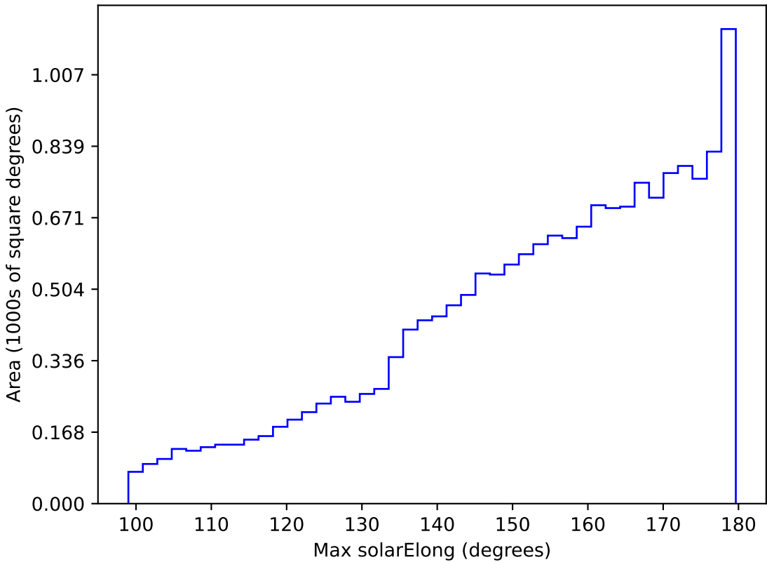
too_elab_r128_d2_gz_v3.4_10yrs WFD all bands: Max solarElong
