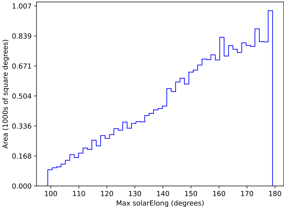
too_elab_r128_d2_gz_v3.4_10yrs All sky y band: Max solarElong
