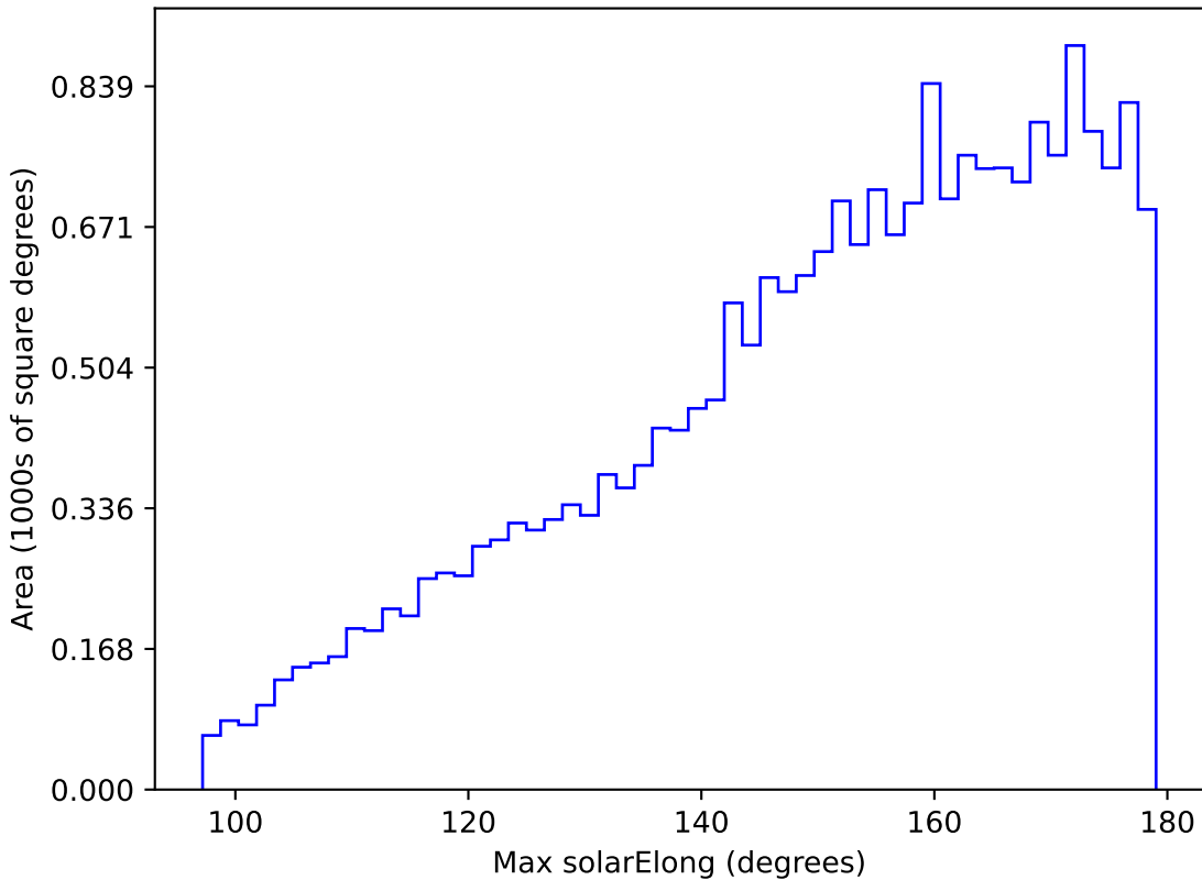
too_elab_r128_d2_gz_v3.4_10yrs All sky u band: Max solarElong
