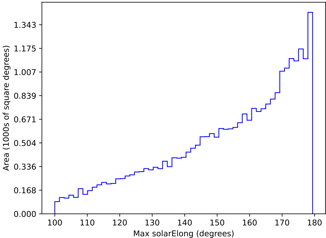
too_elab_r128_d2_gz_v3.4_10yrs All sky i band: Max solarElong
