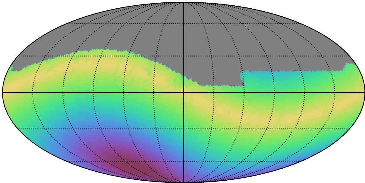
too_elab_r128_d2_gz_v3.4_10yrs All sky g band: Max solarElong
