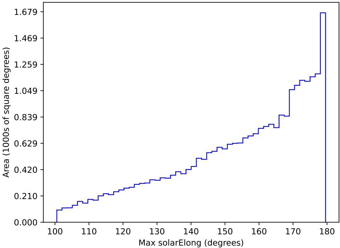
too_elab_r128_d2_gz_v3.4_10yrs All sky all bands: Max solarElong
