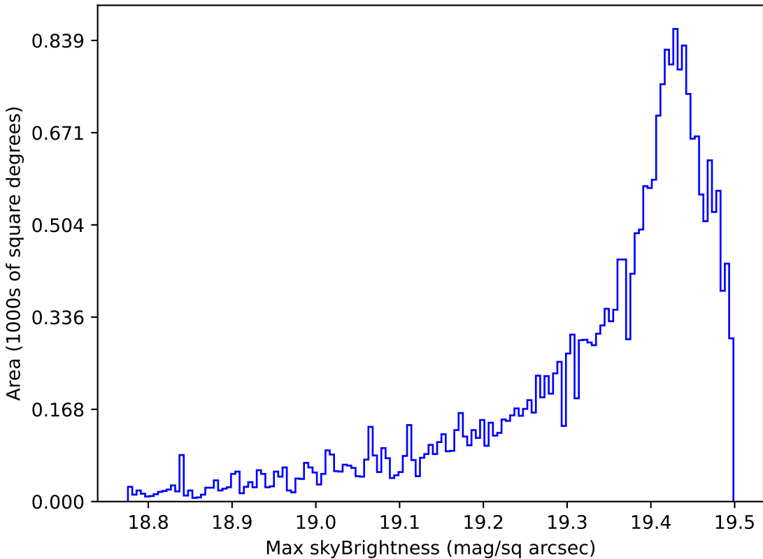
too_elab_r128_d2_gz_v3.4_10yrs Yr 1 z band: Max skyBrightness
