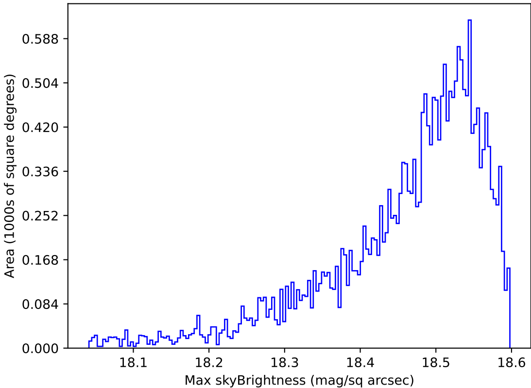
too_elab_r128_d2_gz_v3.4_10yrs Yr 1 y band: Max skyBrightness
