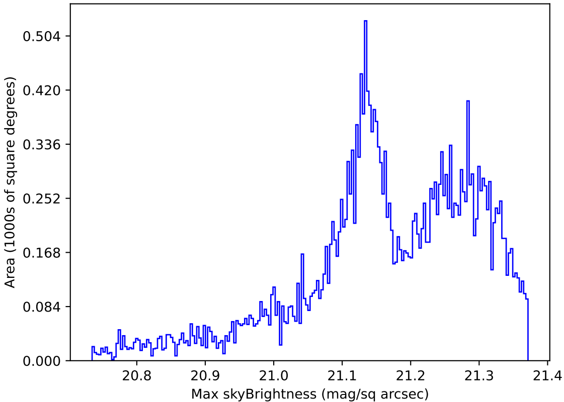
too_elab_r128_d2_gz_v3.4_10yrs Yr 1 r band: Max skyBrightness
