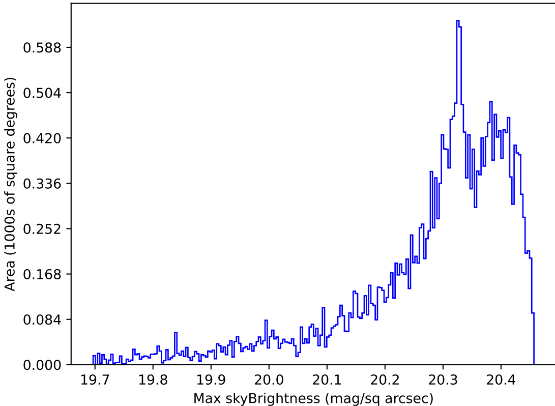
too_elab_r128_d2_gz_v3.4_10yrs Yr 1 i band: Max skyBrightness
