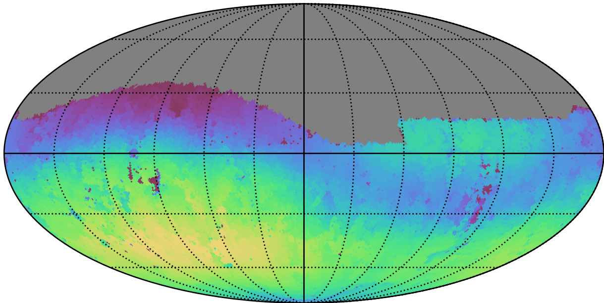
too_elab_r128_d2_gz_v3.4_10yrs Yr 1 g band: Max skyBrightness
