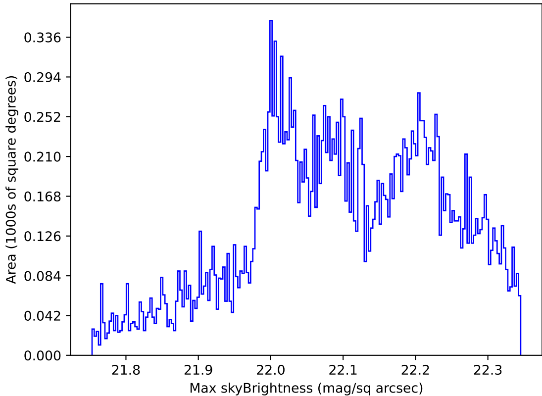
too_elab_r128_d2_gz_v3.4_10yrs Yr 1 g band: Max skyBrightness
