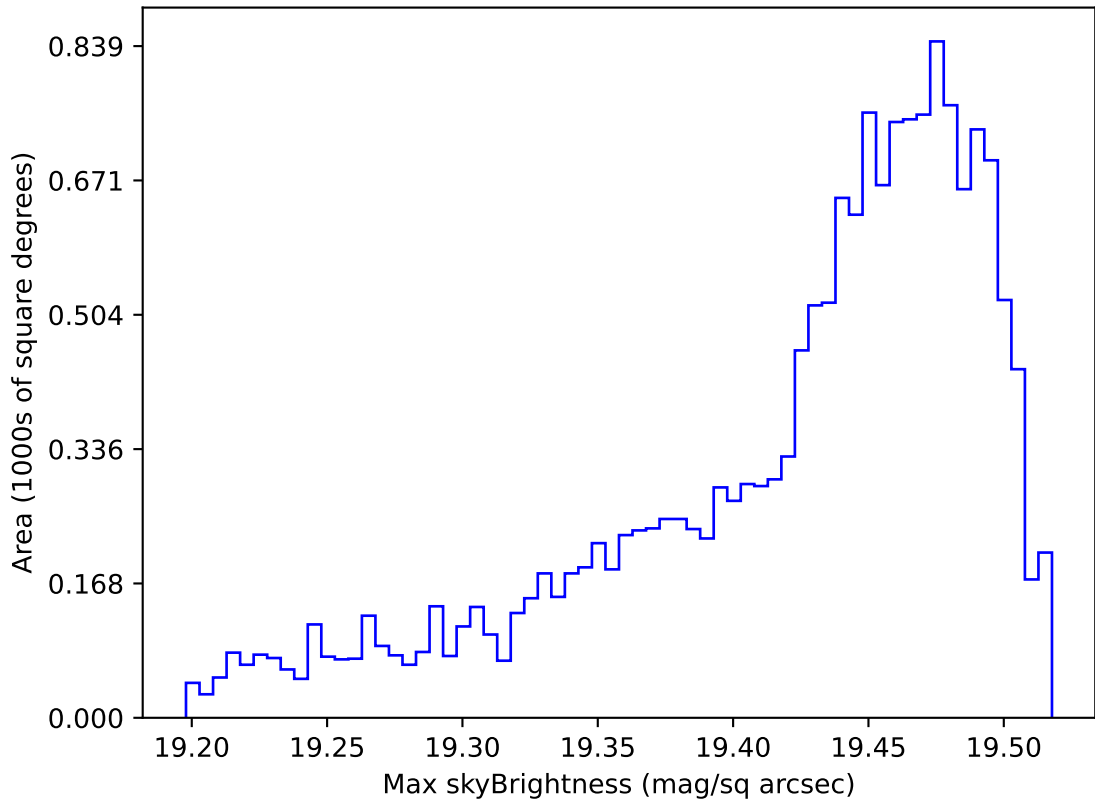
too_elab_r128_d2_gz_v3.4_10yrs WFD z band: Max skyBrightness
