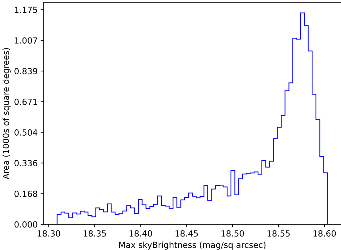
too_elab_r128_d2_gz_v3.4_10yrs WFD y band: Max skyBrightness
