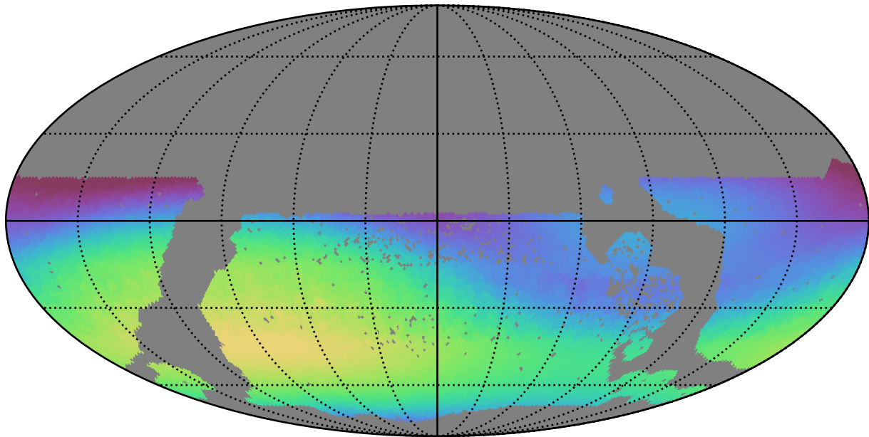
too_elab_r128_d2_gz_v3.4_10yrs WFD r band: Max skyBrightness
