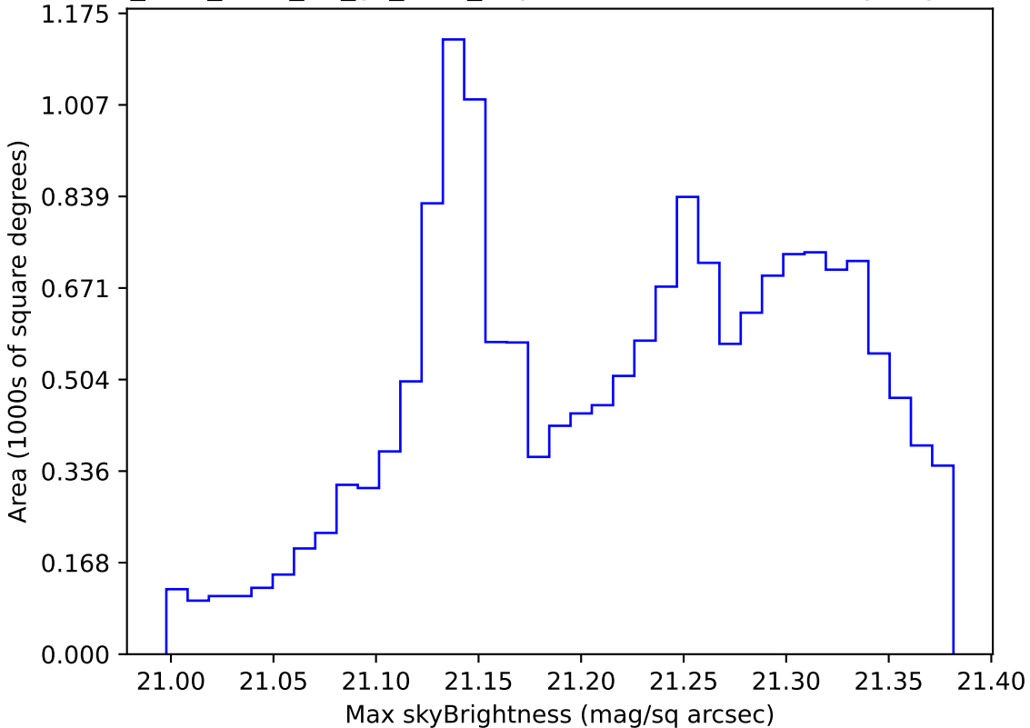
too_elab_r128_d2_gz_v3.4_10yrs WFD r band: Max skyBrightness
