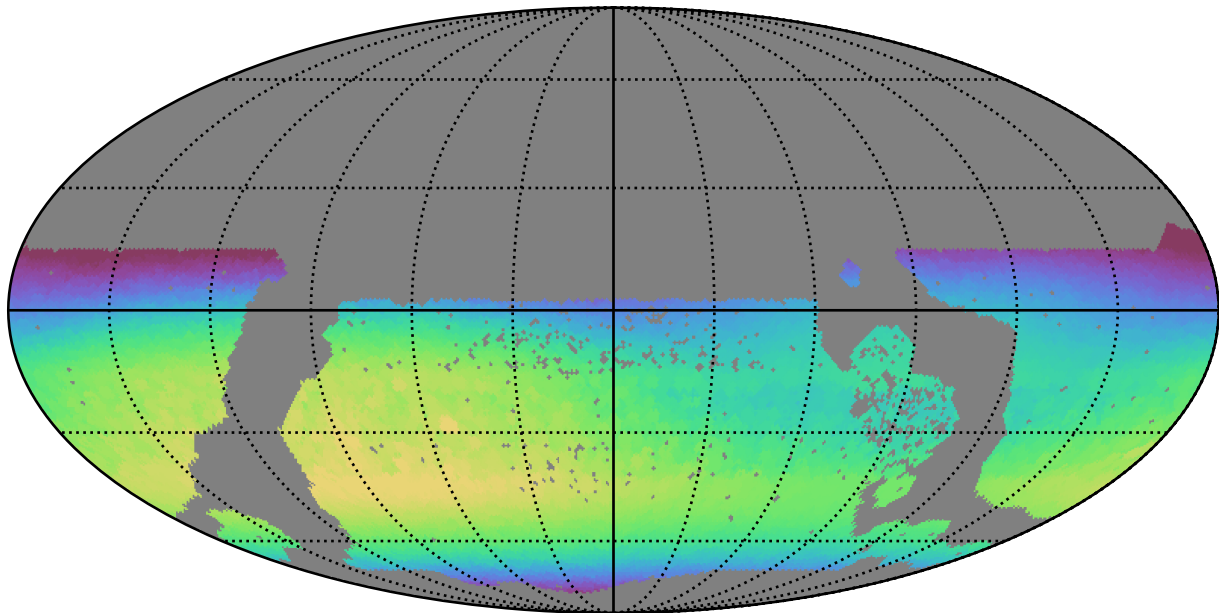
too_elab_r128_d2_gz_v3.4_10yrs WFD i band: Max skyBrightness
