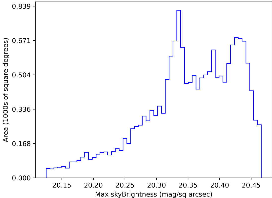
too_elab_r128_d2_gz_v3.4_10yrs WFD i band: Max skyBrightness
