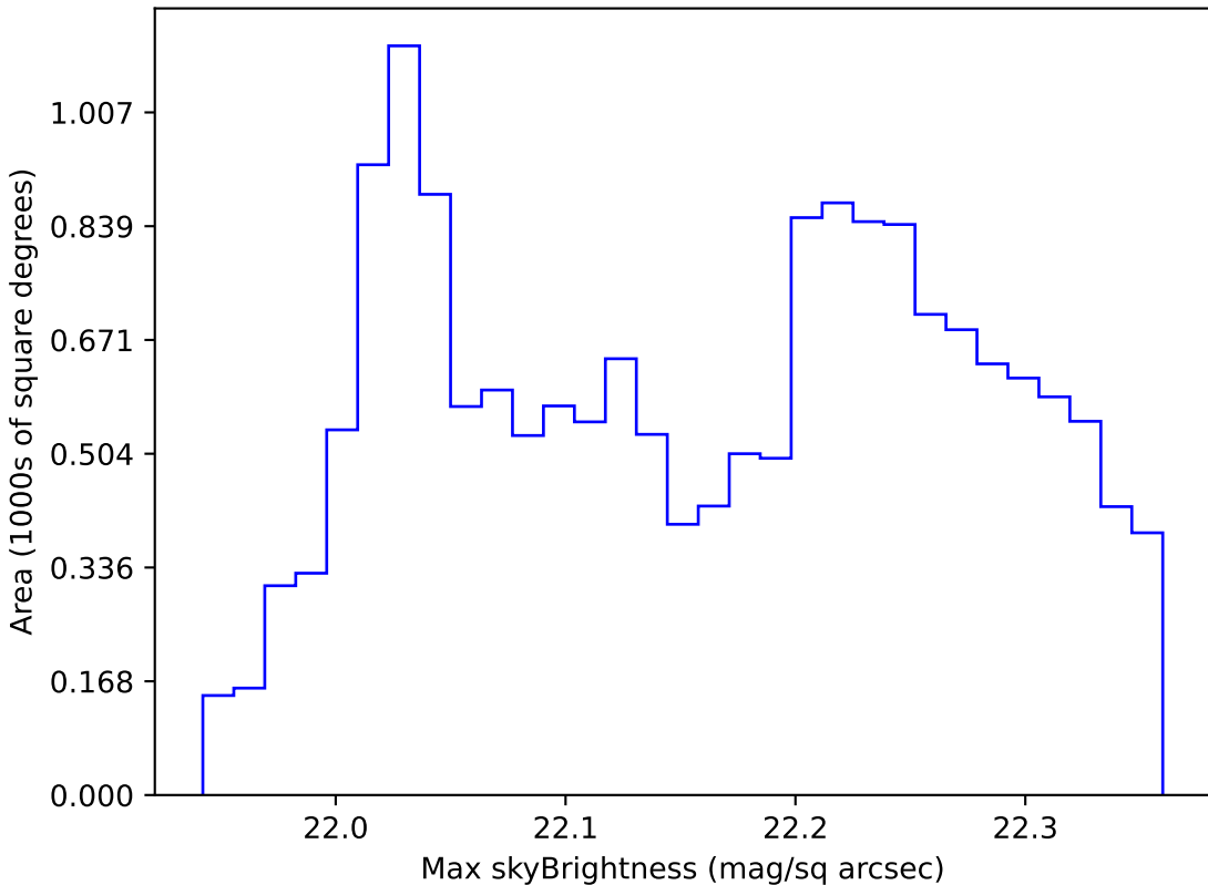
too_elab_r128_d2_gz_v3.4_10yrs WFD g band: Max skyBrightness
