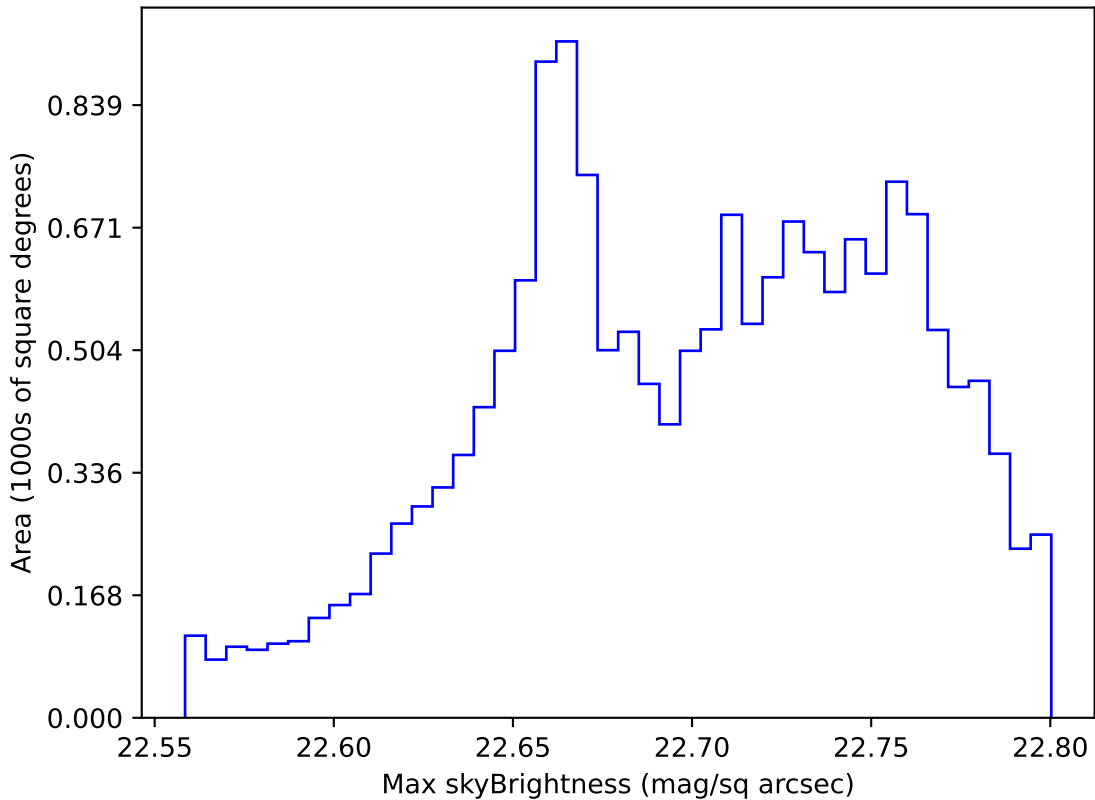
too_elab_r128_d2_gz_v3.4_10yrs WFD all bands: Max skyBrightness
