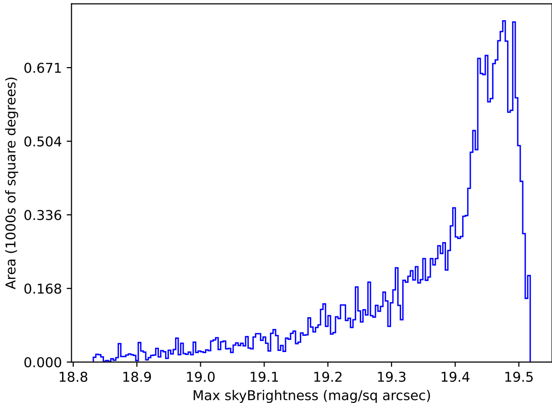
too_elab_r128_d2_gz_v3.4_10yrs All sky z band: Max skyBrightness
