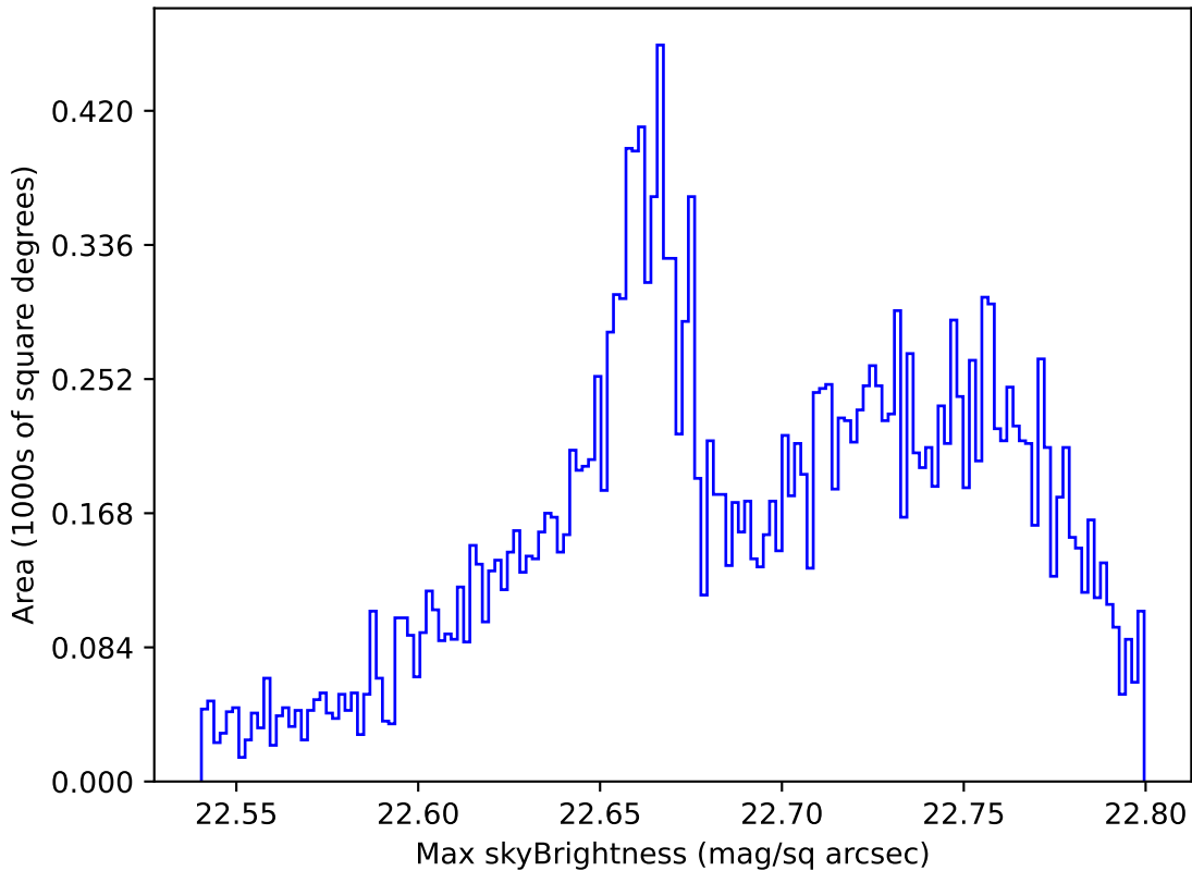
too_elab_r128_d2_gz_v3.4_10yrs All sky u band: Max skyBrightness
