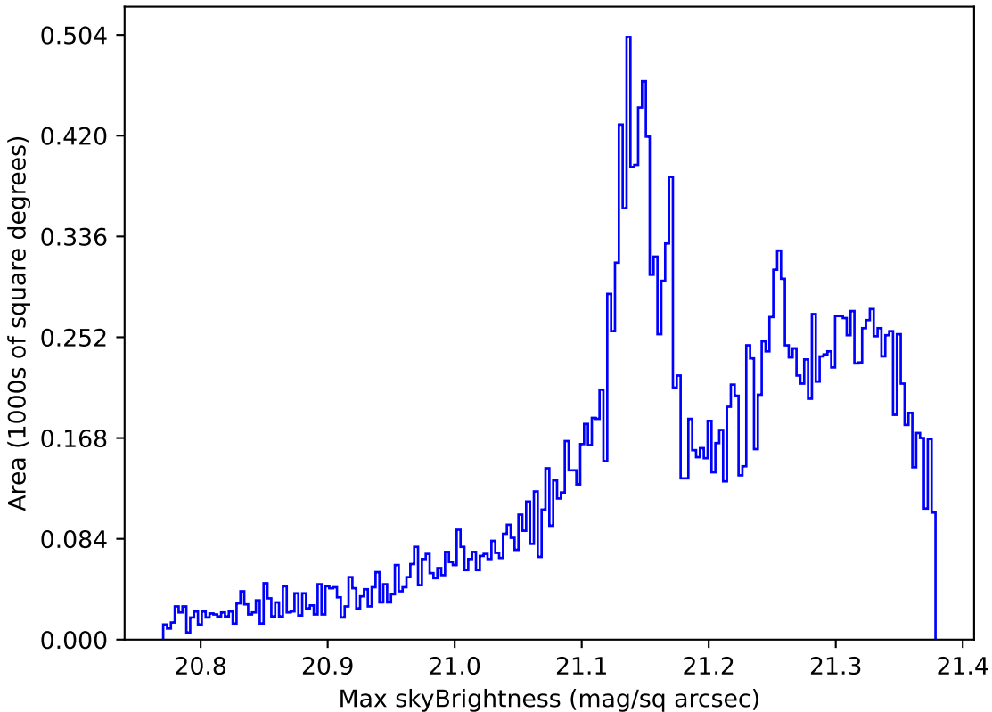
too_elab_r128_d2_gz_v3.4_10yrs All sky r band: Max skyBrightness
