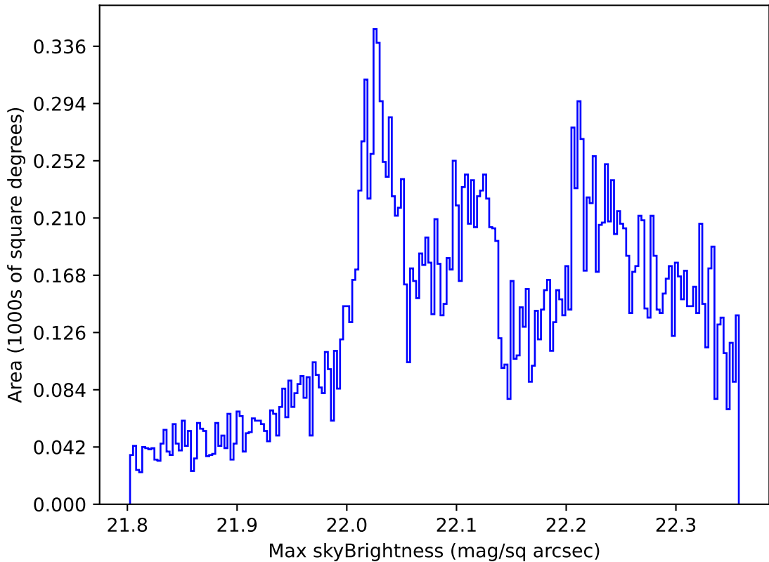
too_elab_r128_d2_gz_v3.4_10yrs All sky g band: Max skyBrightness
