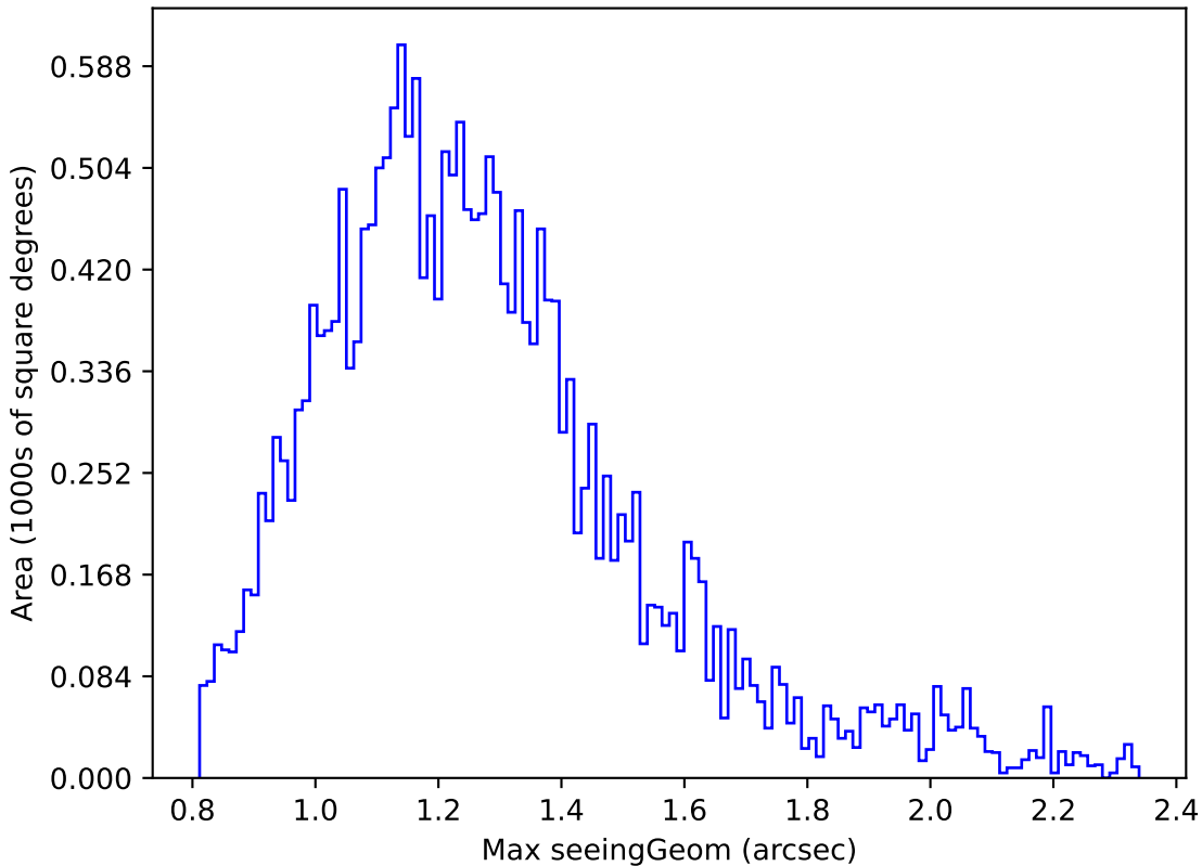
too_elab_r128_d2_gz_v3.4_10yrs Yr 1 y band: Max seeingGeom
