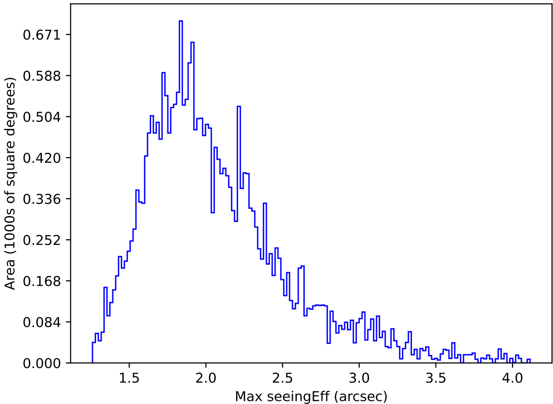
too_elab_r128_d2_gz_v3.4_10yrs Yr 1 all bands: Max seeingEff
