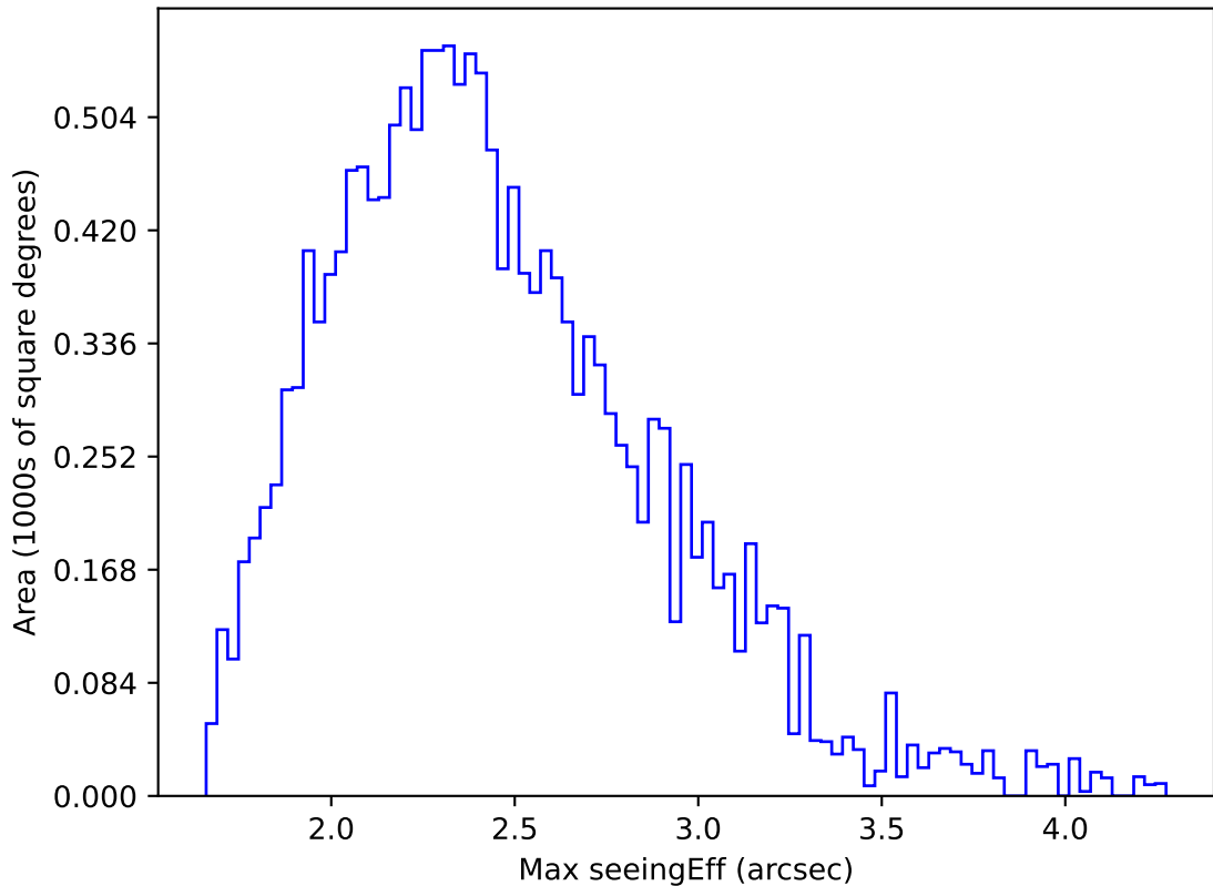
too_elab_r128_d2_gz_v3.4_10yrs WFD z band: Max seeingEff
