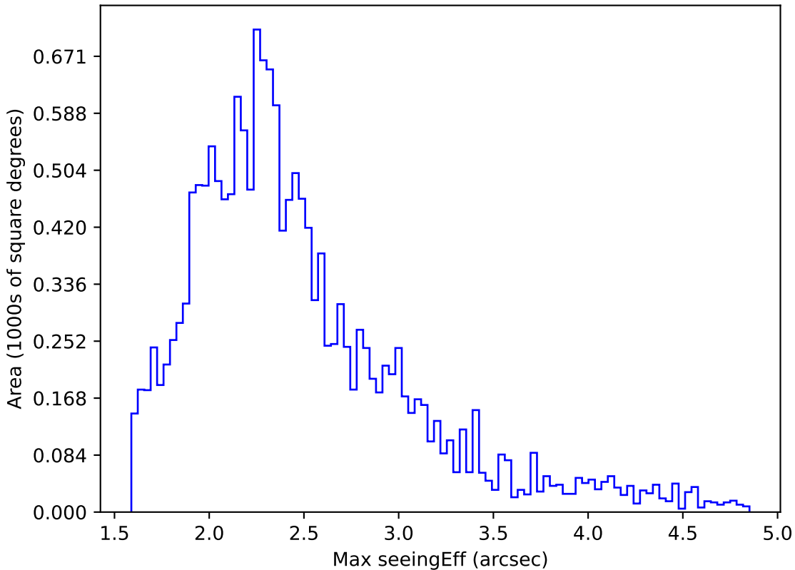
too_elab_r128_d2_gz_v3.4_10yrs WFD y band: Max seeingEff
