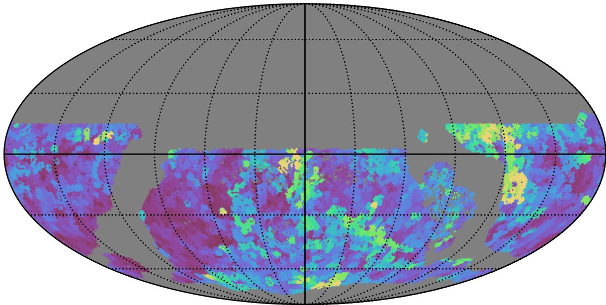
too_elab_r128_d2_gz_v3.4_10yrs WFD r band: Max seeingEff
