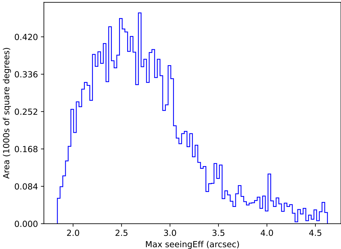
too_elab_r128_d2_gz_v3.4_10yrs WFD r band: Max seeingEff
